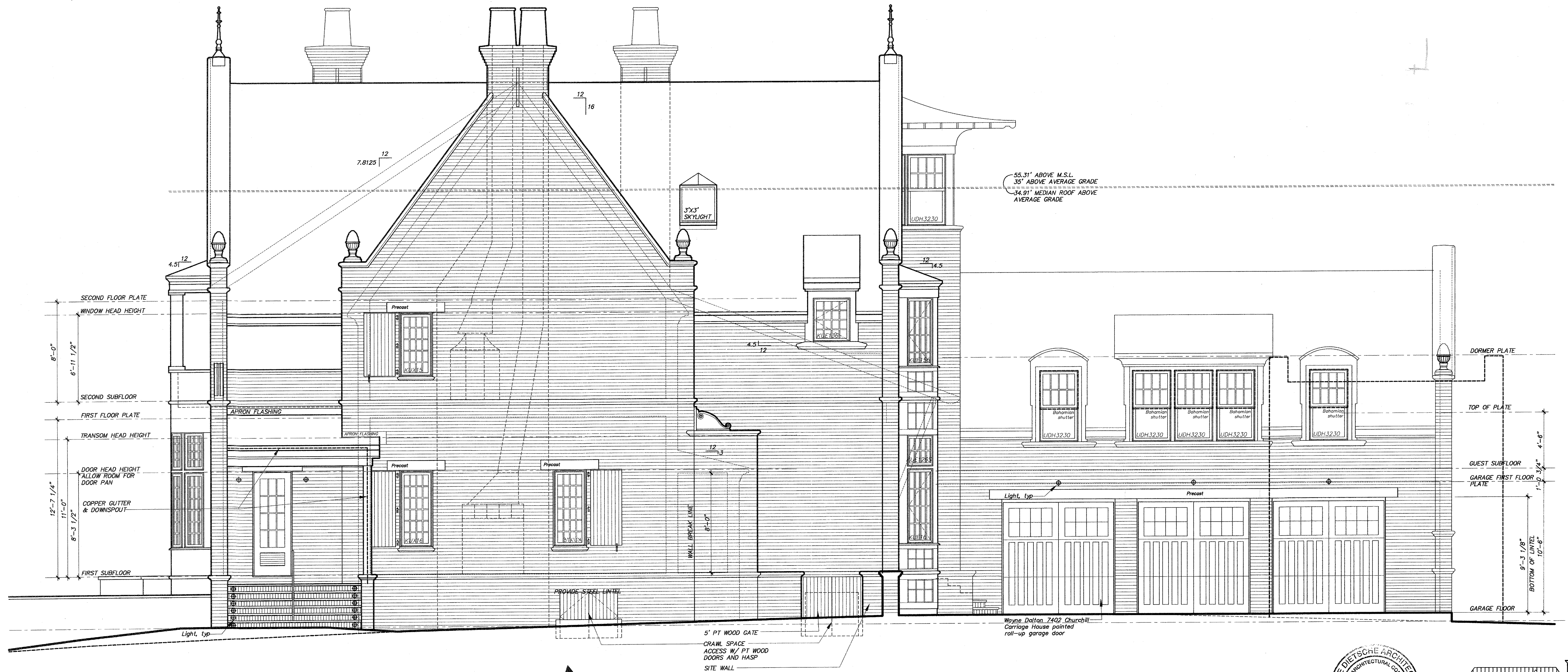
1 a13 Left Elevation 1/4"=1'-0"
