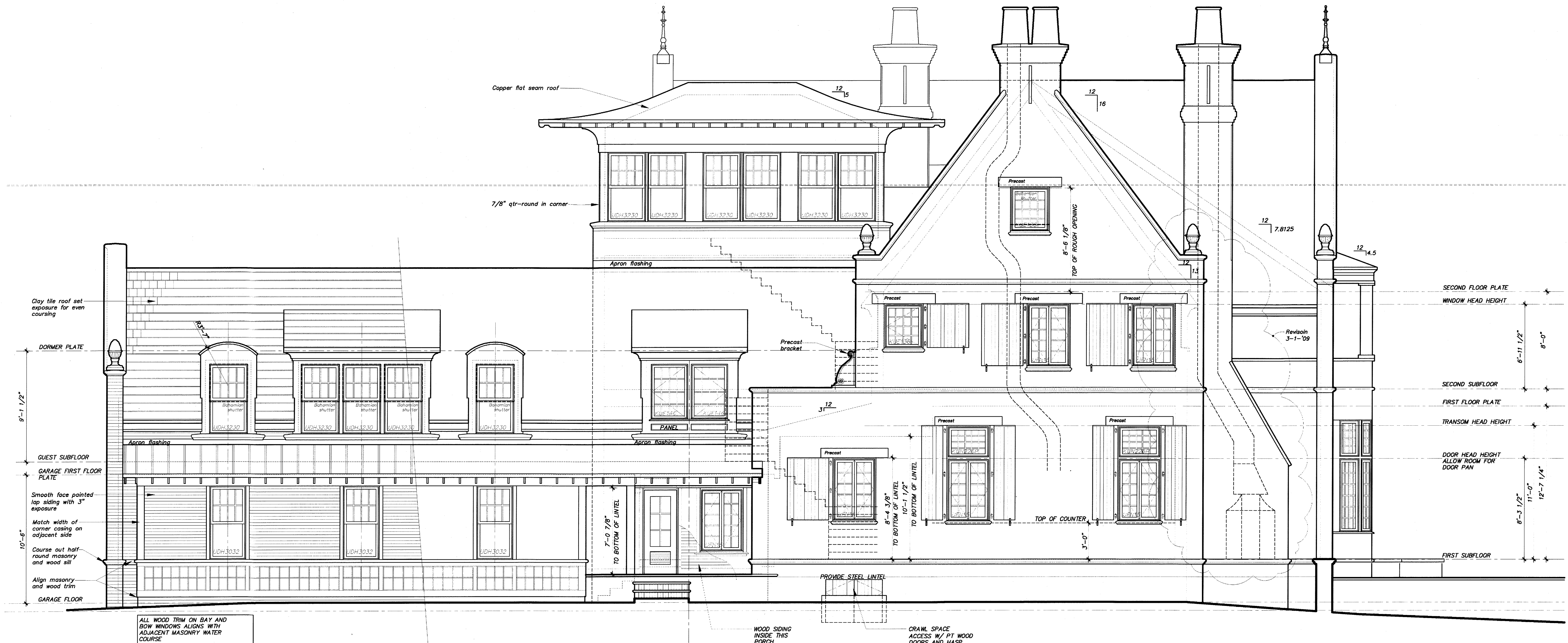
1 a12 Right Elevation 1/4" = 1'-0"
