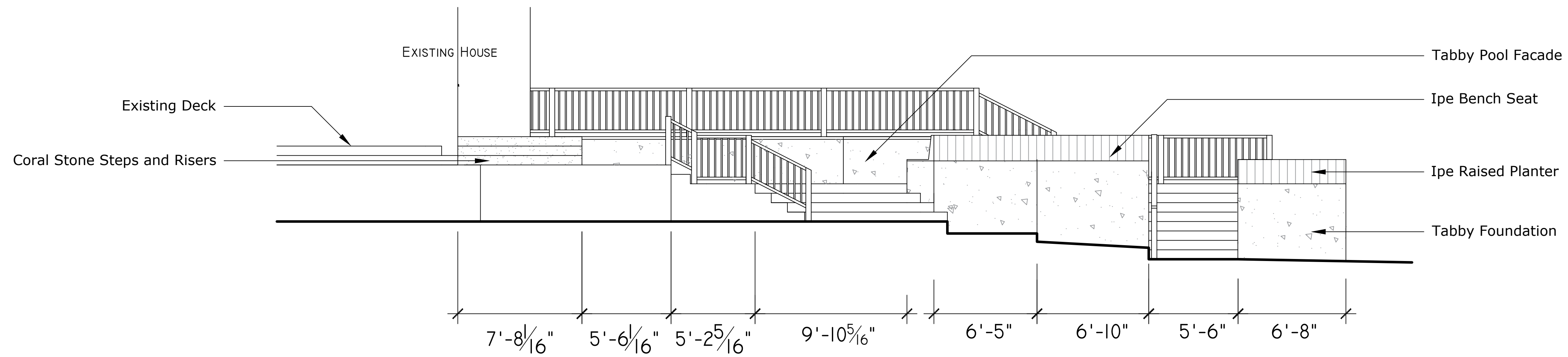
Left Elevation
