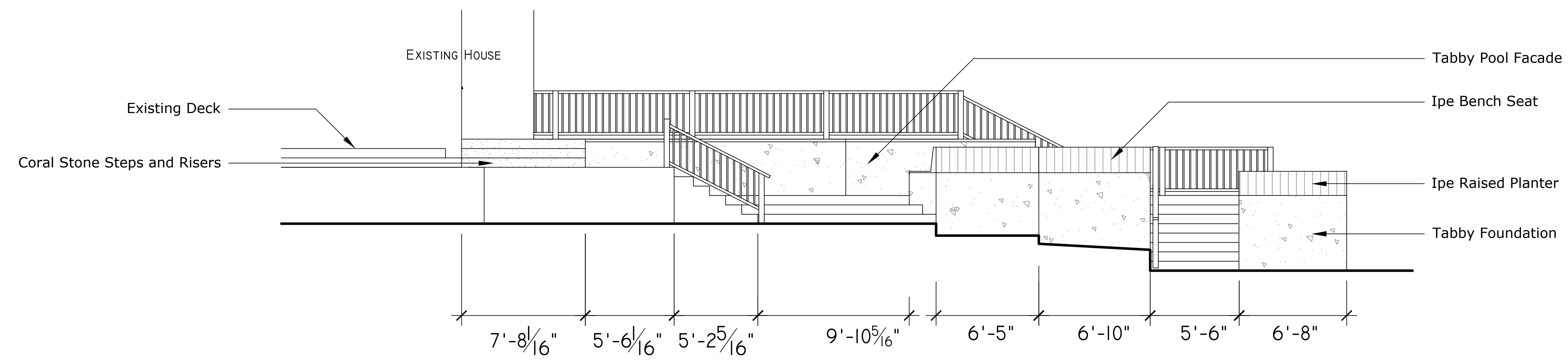
Left Elevation
